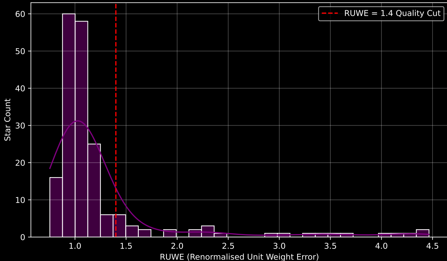
GAPOGEE DR17 Field [K2_C12_082-57_btx] RUWE Distribution (n= 195)
