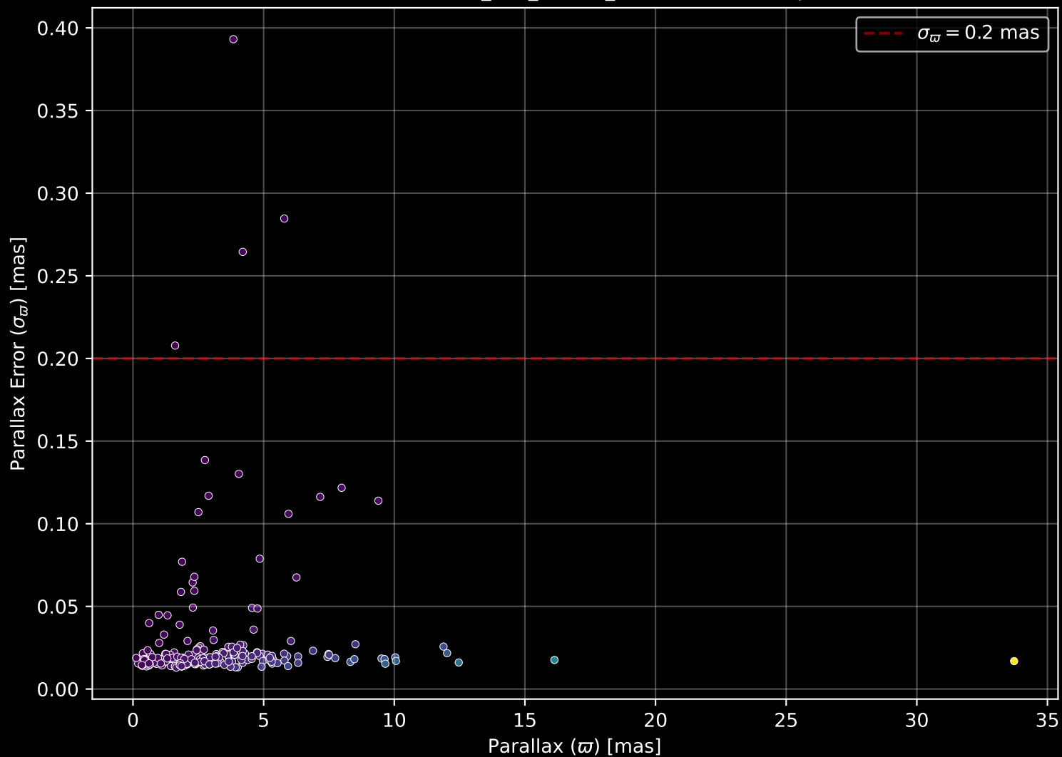
APOGEE DR17 Field: [K2_C12_082-57_btx] Parallax Quality (n= 205)
