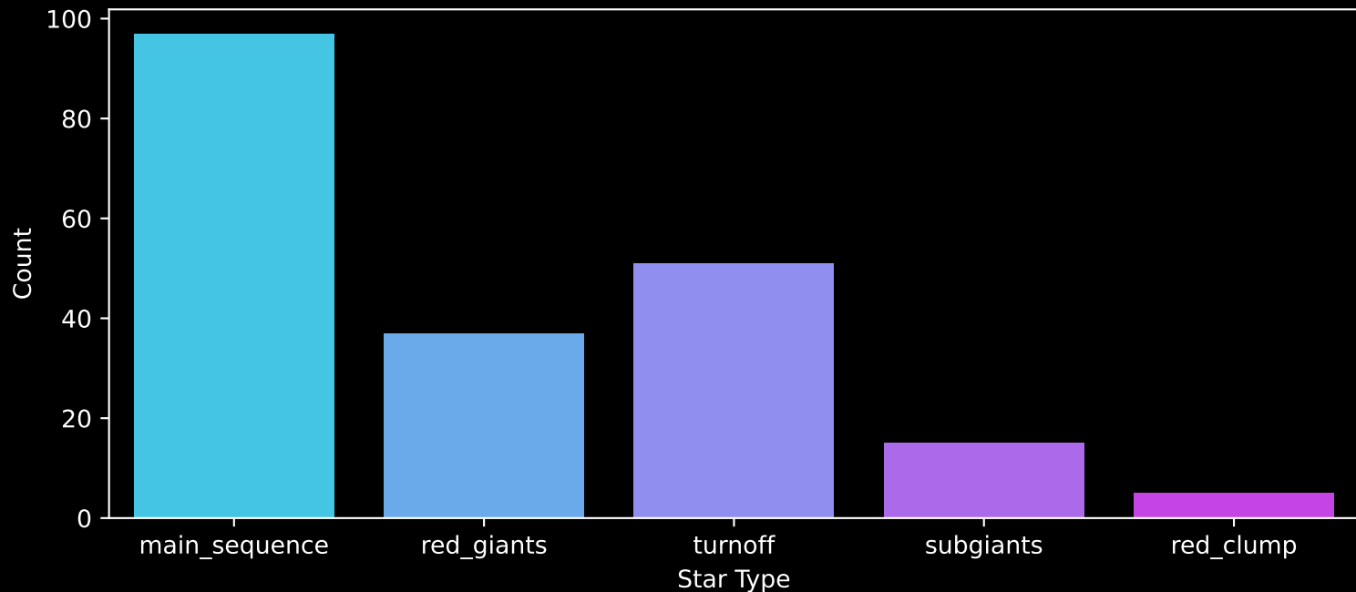
APOGEE DR17 Field: [K2_C12_082-57_btx] Count plot of Star Type
