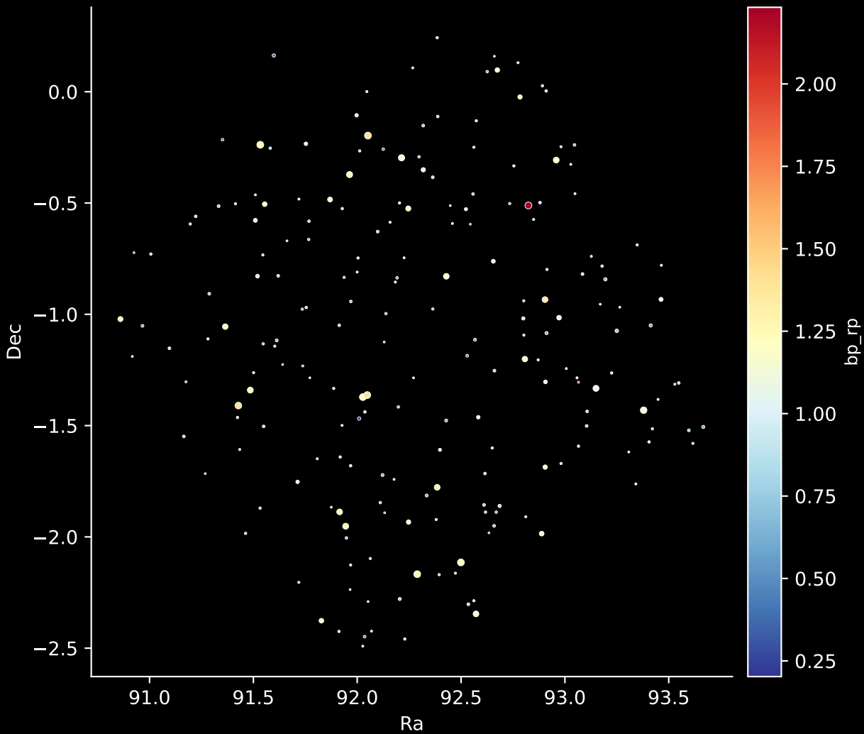
APOGEE DR17 Field: [K2_C12_082-57_btx] Stars: 205
