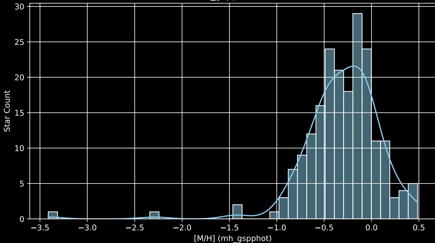
APOGEE DR17 Field: [K2_C12_082-57_btx [M/H] (mh_gspphot) (n= 202)
