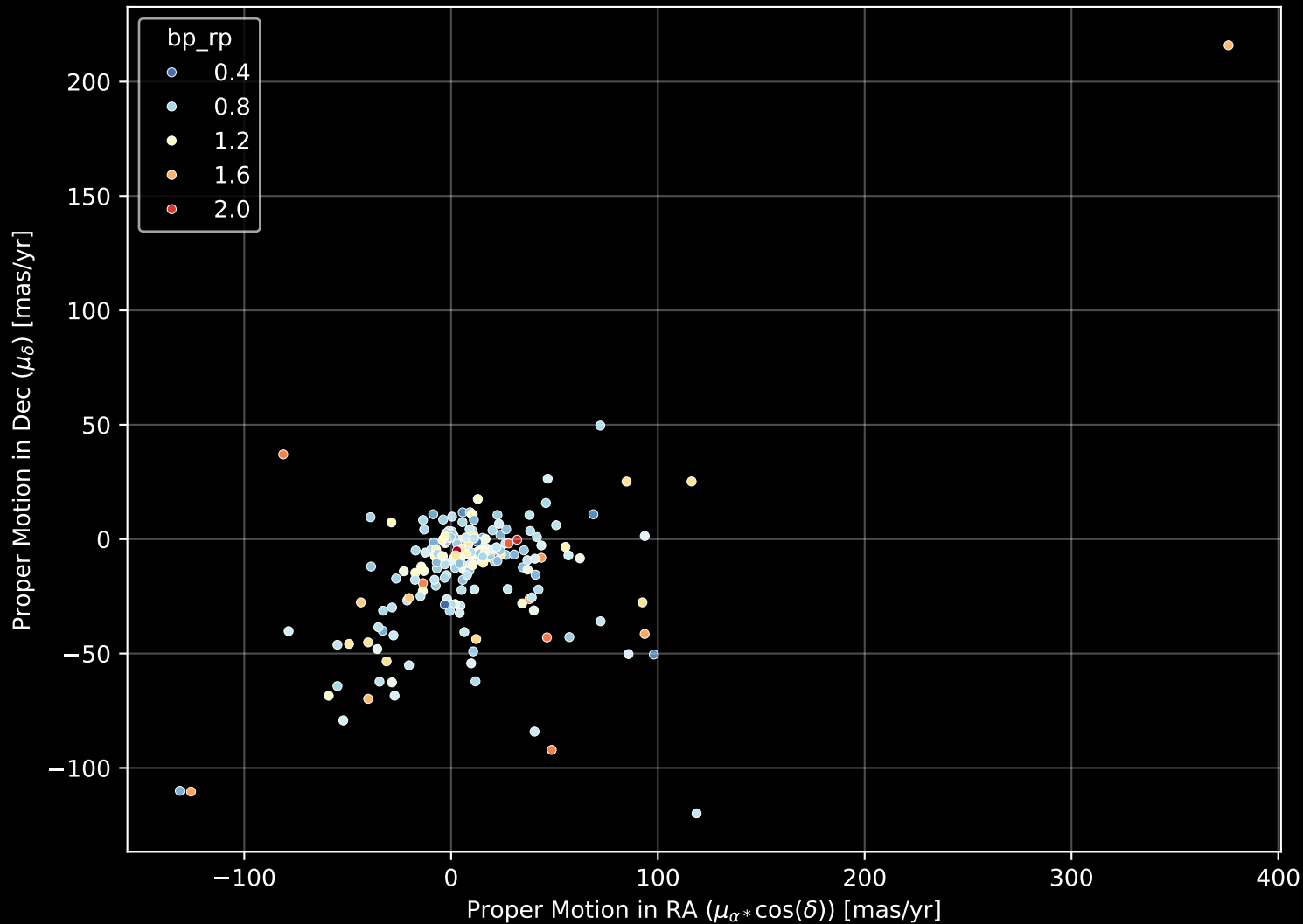
APOGEE DR17 Field: [K2_C12_082-57_btx] Proper Motion Diagram (n= 205)
